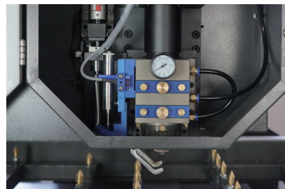
Laser head
